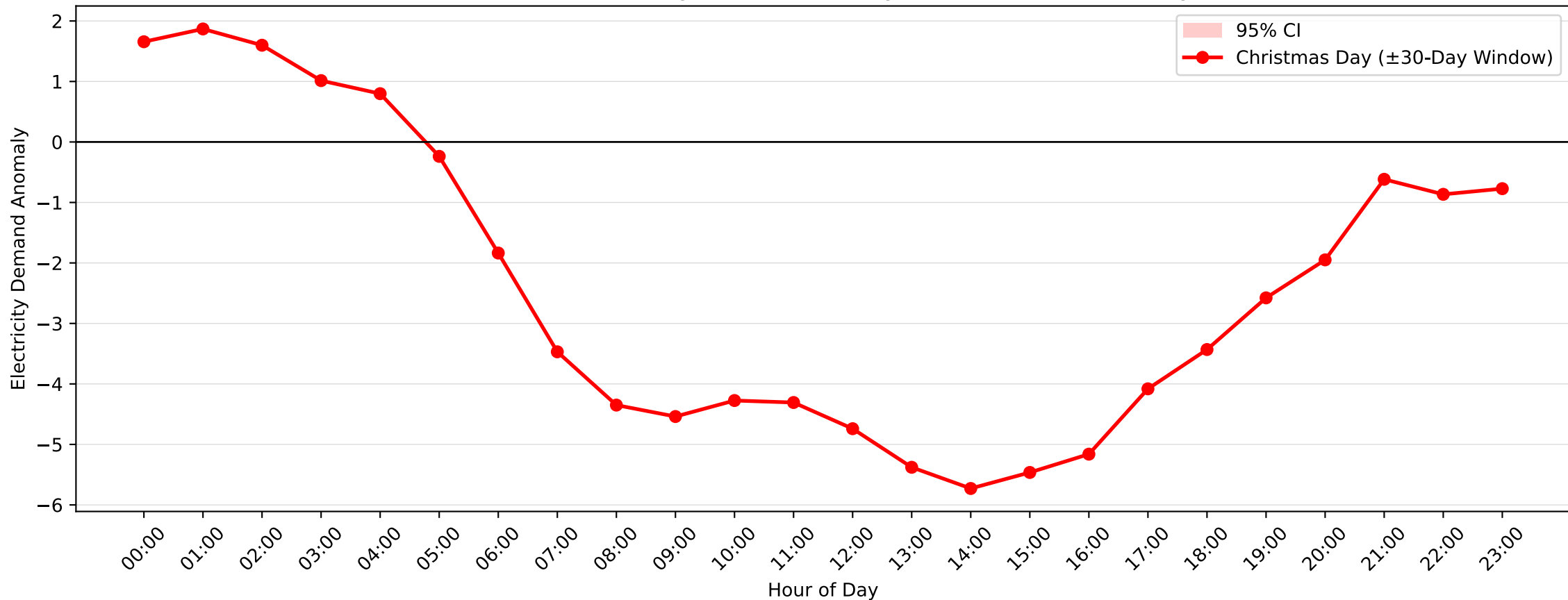
Maroubra Demand Anomaly: Christmas Day (2016-2017, \pm 30 -Day Window)
