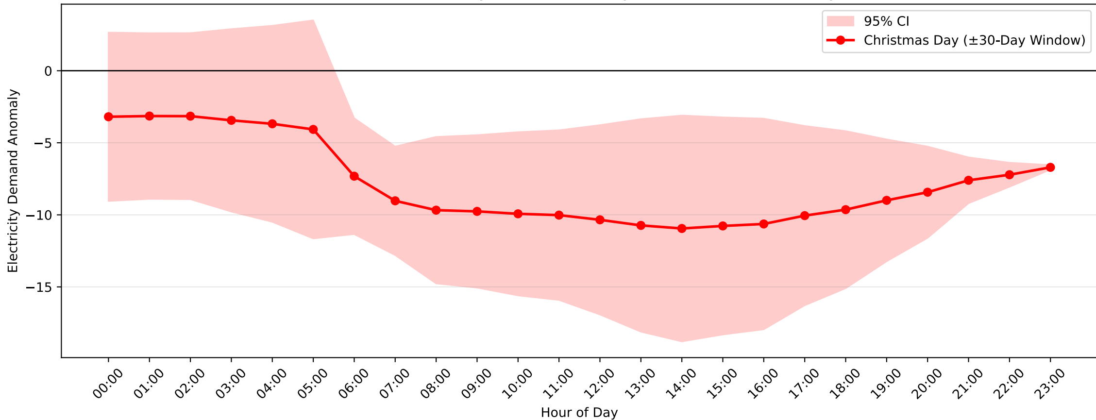
Maroubra Demand Anomaly: Christmas Day (2014-2015, \pm 30 -Day Window)
