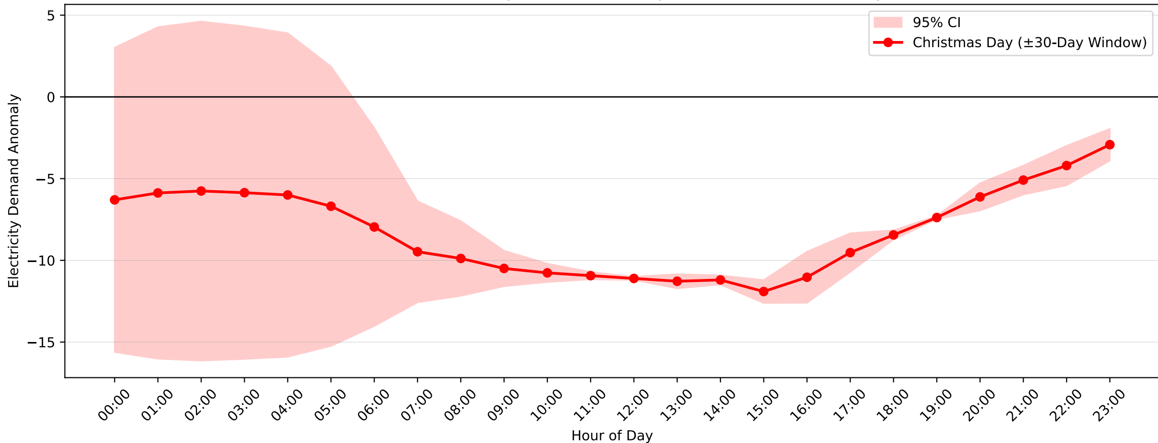
Maroubra Demand Anomaly: Christmas Day (2008-2009, \pm 30 -Day Window)
